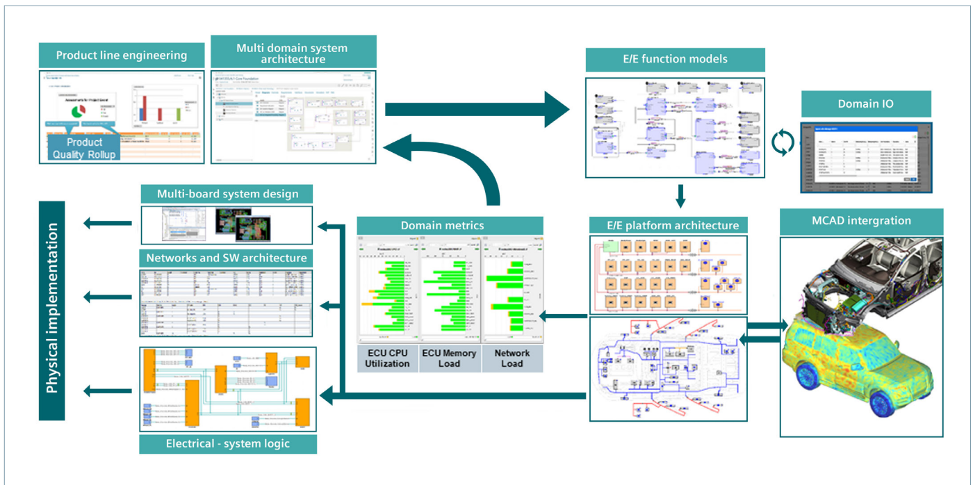
Figure 4: A full flow from system design to E/E implementation.
