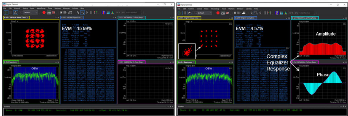
Figure 5. Simulation results with bandpass filter and power amplifier added
