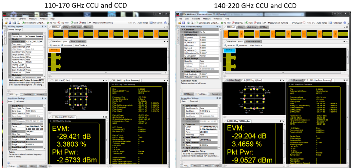
Figure 8. 16 QAM MCS12 measurements performed at 144 GHz with D-band (left) and G-band (right) VDI converters, CB4 configuration with 8.64 GHz channel bandwidth
