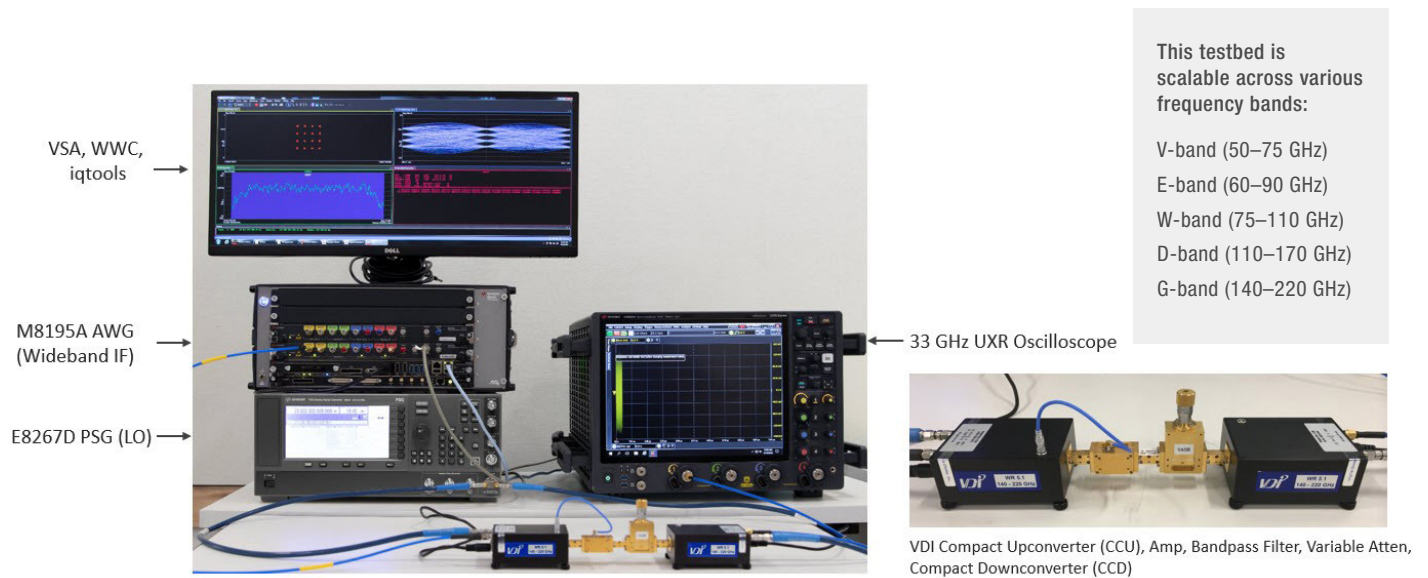
Figure 6. Sub-terahertz R&D testbed, conducted measurements
