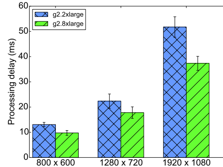
Fig. 5: Average processing delay as a function of the resolution for different Amazon GPU instances.
