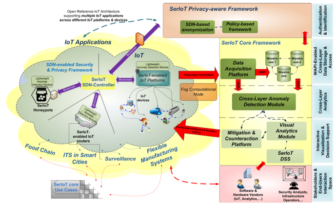
Fig. 1: Overview of SerIoT’s architecture.
